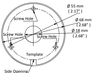
Figure 2-8 Drill Template
